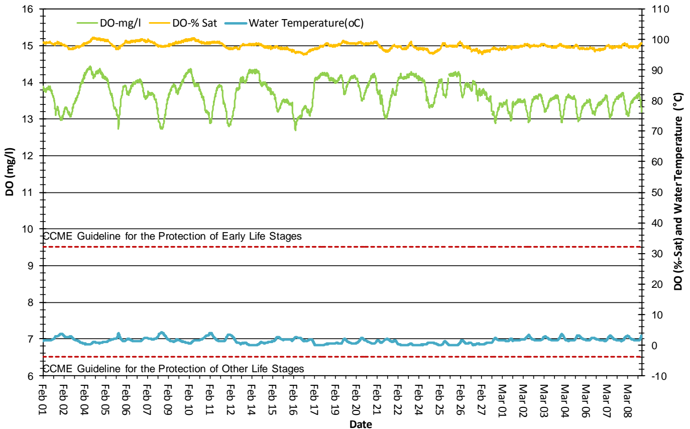
Dissolved Oxygen Concentration and Saturation at Leary's Brook
