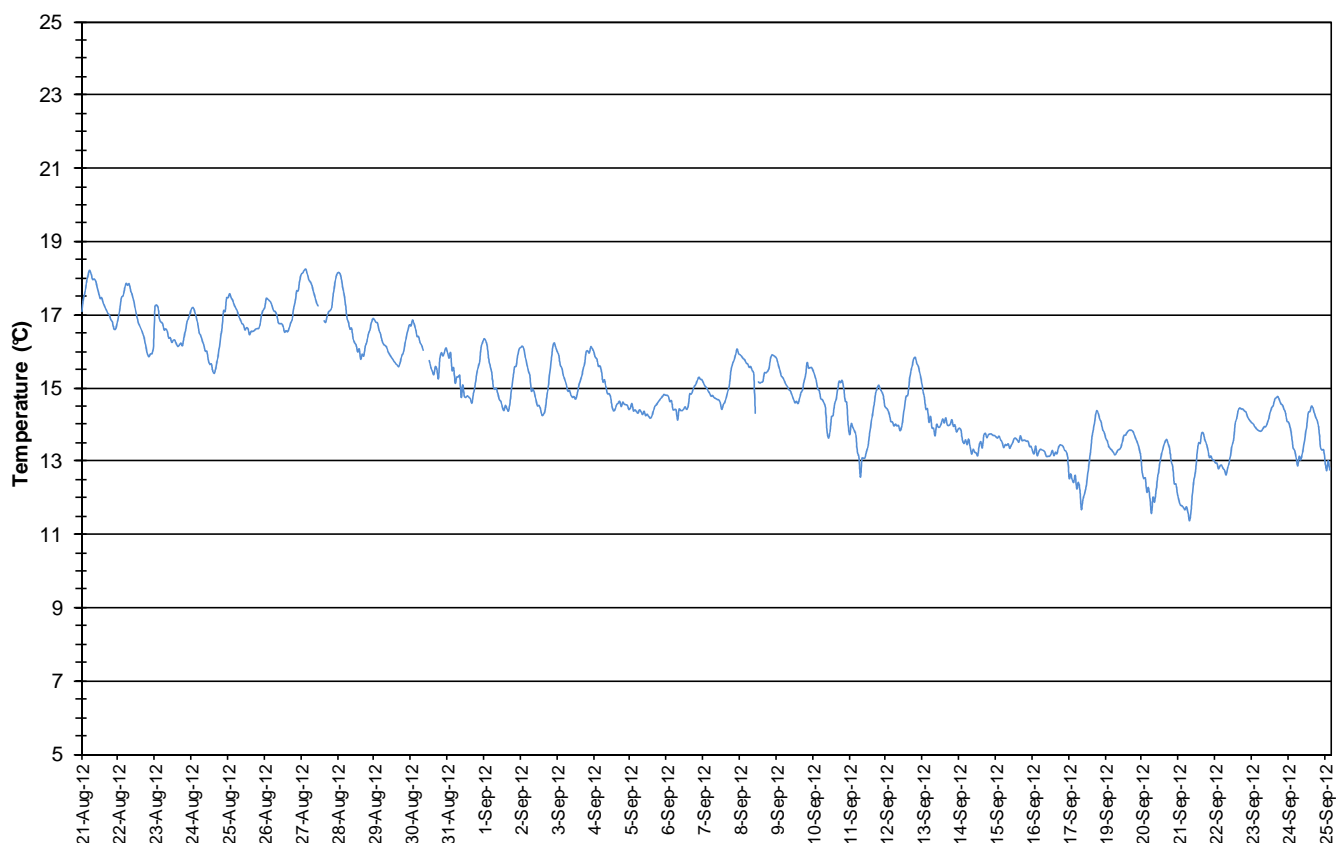
Water Temperature: Minipi River below Minipi Lake August 21 to September 25, 2012
