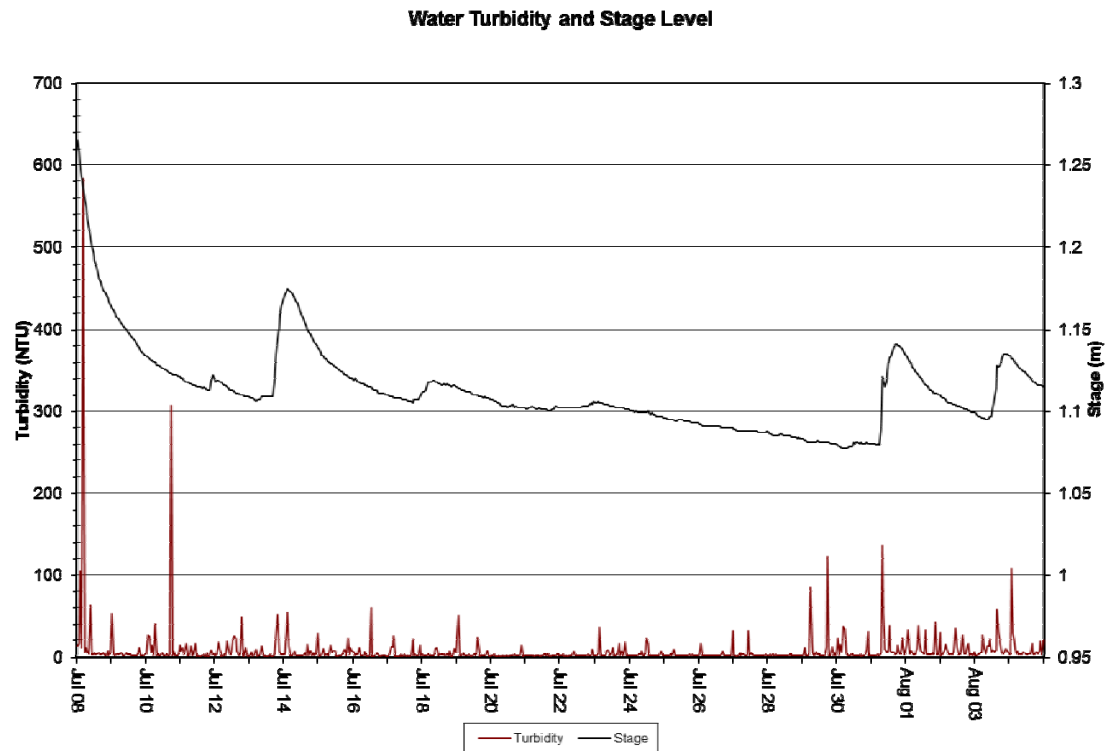
Figure 11: Turbidity (NTU) at Elross Creek – July 8, 2015 to August 5, 2015
