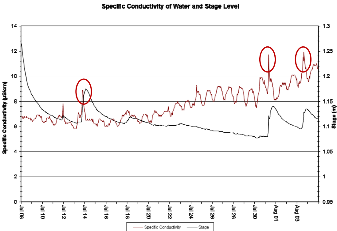
Figure 7: Specific conductivity (us/cm) - Elross Creek – July 8, 2015 to August 5, 2015
