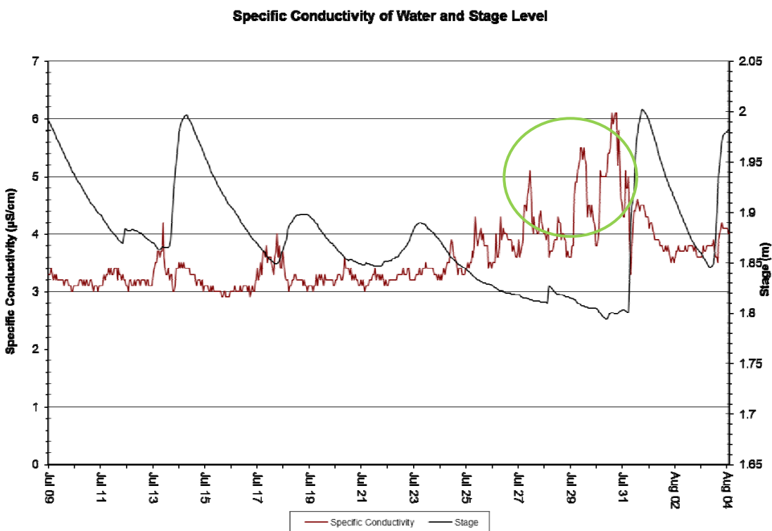
Figure 8: Specific conductivity (us/cm) - Goodream Creek – July 9, 2015 to August 4, 2015
