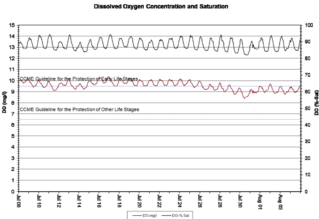
Figure 9: DO (mg/l & % saturation) at Elross Creek – July 8, 2015 to August 5, 2015
