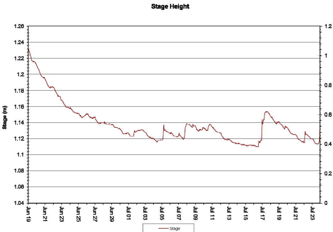
Figure 1: Stage Height (m) at Elross Creek – June 19, 2018 to July 24, 2018
