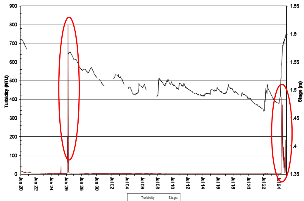
Figure 12: Turbidity (NTU) at Joan Brook – June 20, 2018 to July 25, 2018
