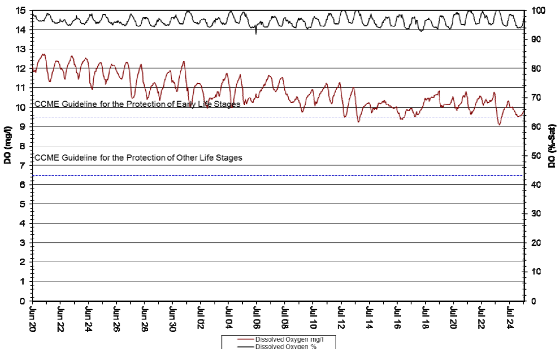
Figure 10: DO (mg/l & % Sat.) at Joan Brook – June 20, 2018 to July 25, 2018
