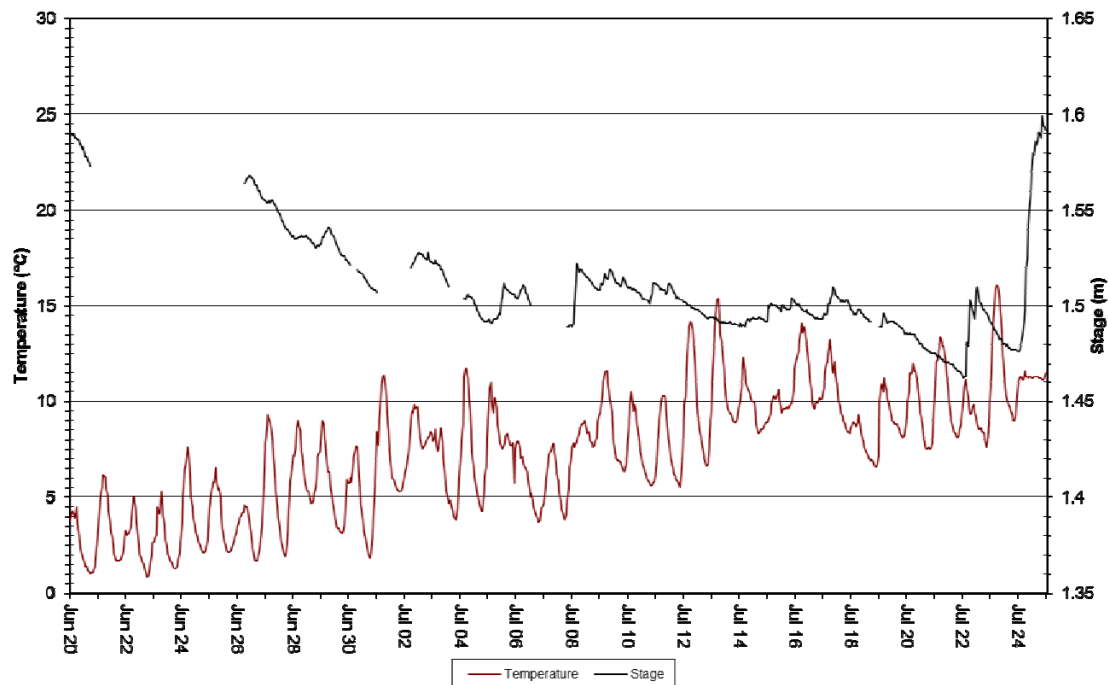
Figure 4: Temperature (°C) – Joan Brook – June 20, 2018 to July 25, 2018
