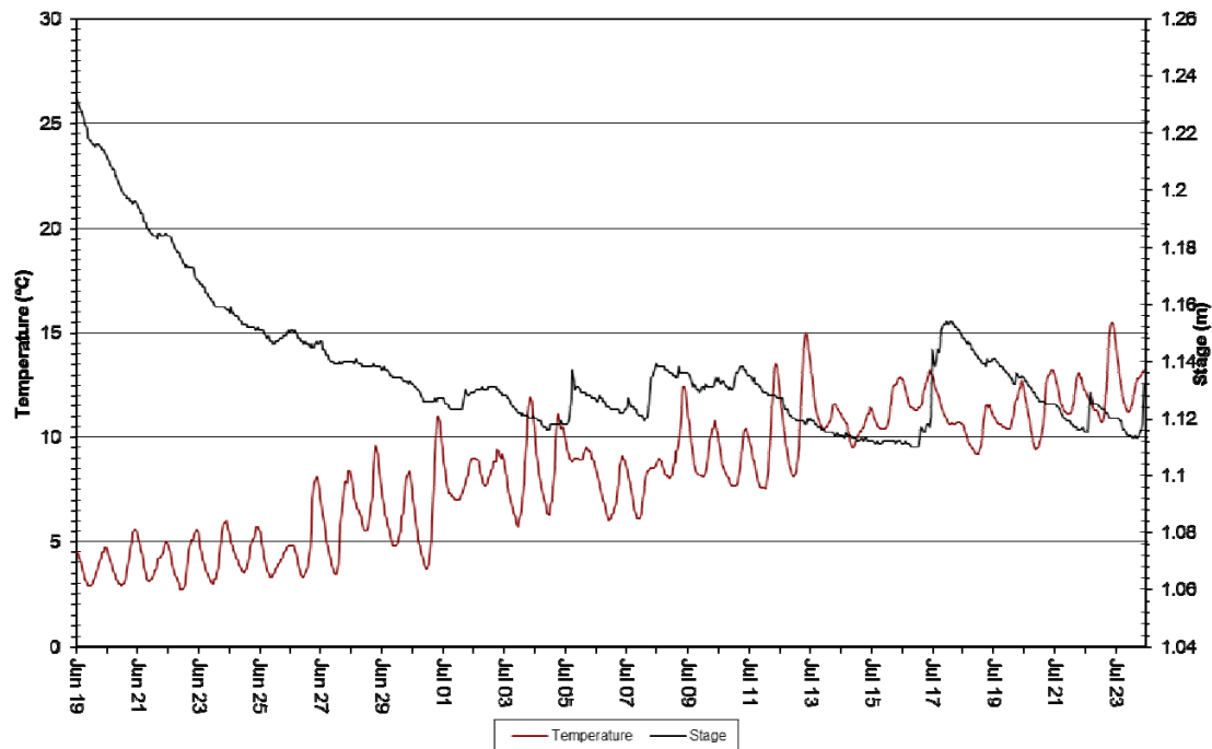
Figure 3: Temperature (°C) - Elross Creek – June 19, 2018 to July 24, 2018
