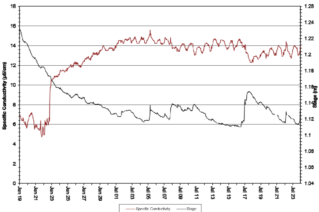
Figure 7: Specific Conductivity at Elross Creek – June 19, 2018 to July 24, 2018
