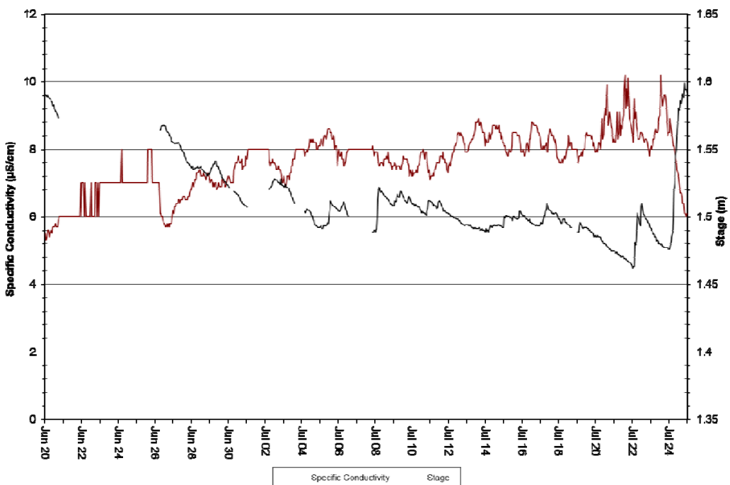
Figure 8: Specific Conductivity at Joan Brook – June 20, 2018 to July 25, 2018
