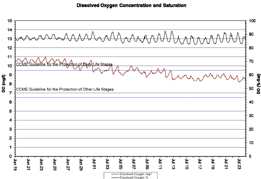
Figure 9: DO (mg/l & % Sat.) at Elross Creek – June 19, 2018 to July 24, 2018
