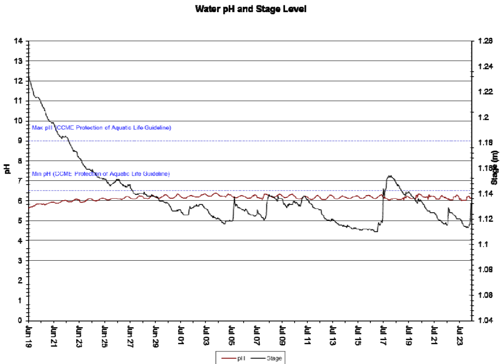
Figure 5: pH at Elross Creek – June 19, 2018 to July 24, 2018
