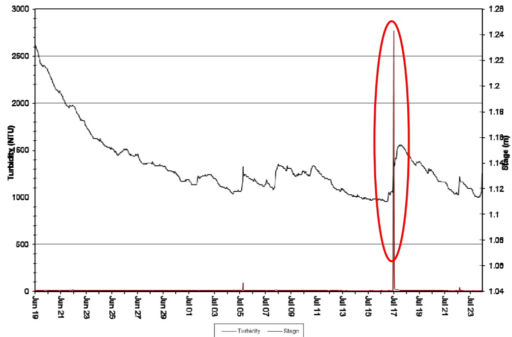
Figure 11: Turbidity (NTU) at Elross Creek – June 19, 2018 to July 24, 2018
