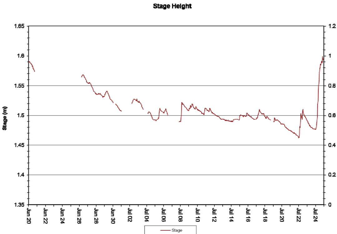
Figure 2: Stage Height (m) at Joan Brook – June 20, 2018 to July 25, 2018
