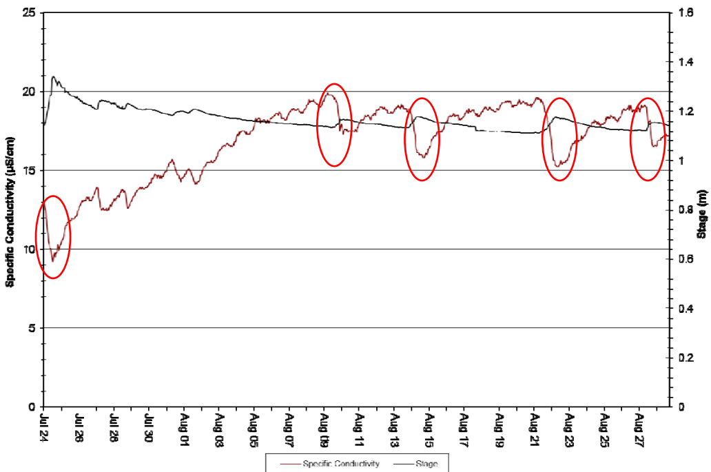
Figure 7: Specific Conductivity at Elross Creek – July 24, 2018 to August 29, 2018
