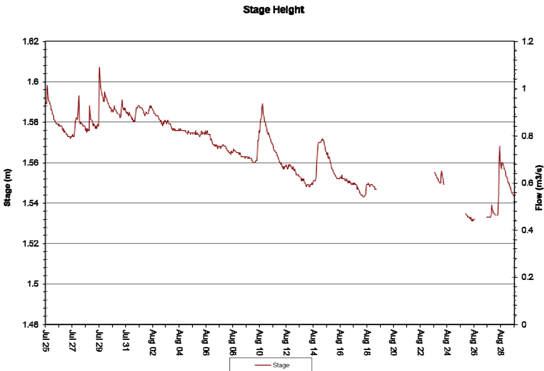
Figure 2: Stage Height (m) at Joan Brook – July 25, 2018 to August 29, 2018
