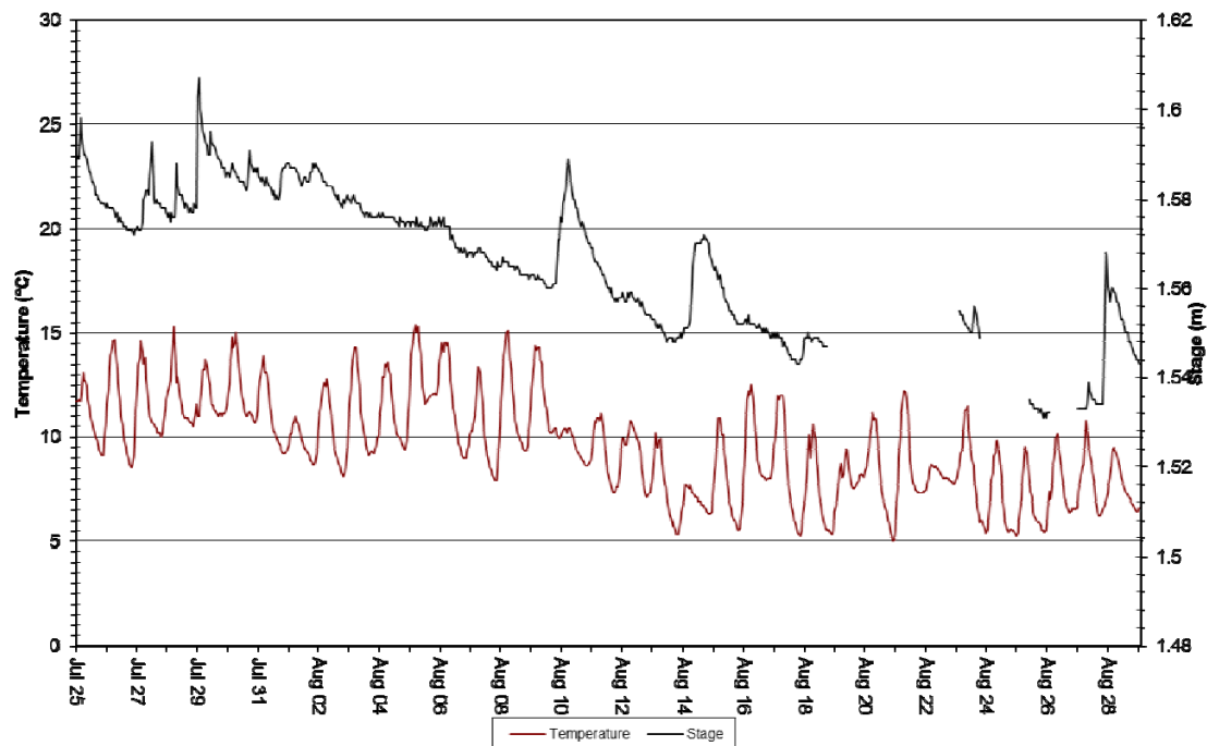
Figure 4: Temperature (°C) – Joan Brook – July 25, 2018 to August 29, 2018
