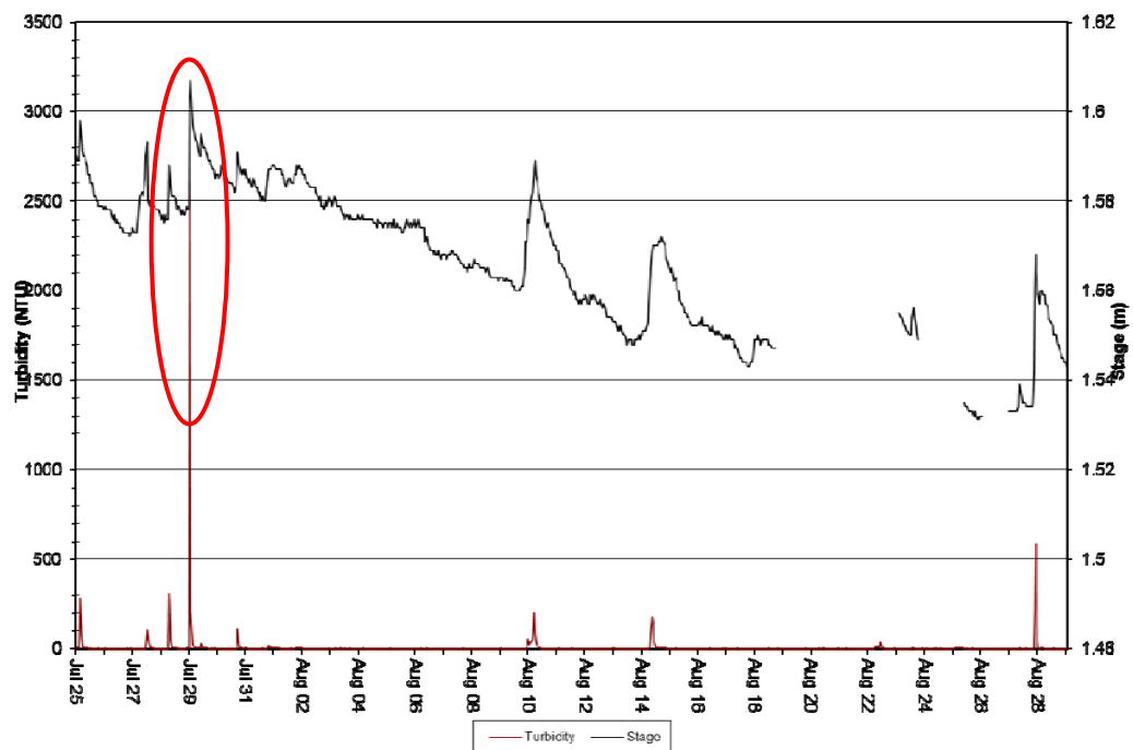
Figure 12: Turbidity (NTU) at Joan Brook – July 25, 2018 to August 29, 2018
