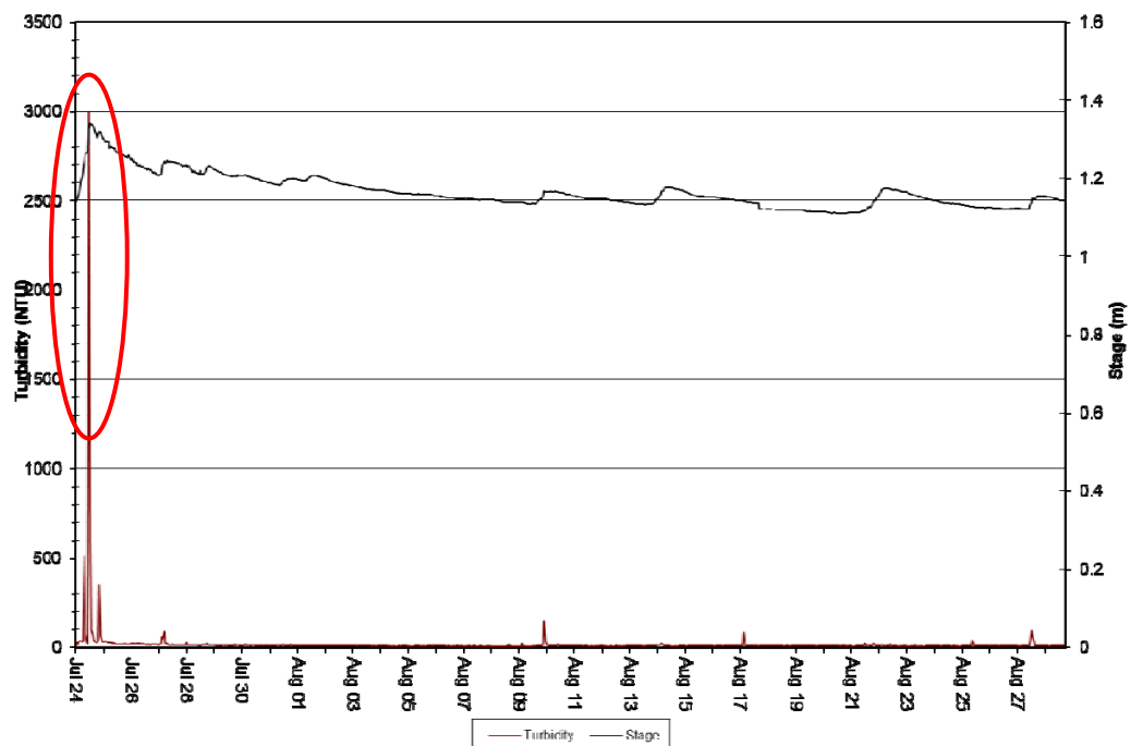
Figure 11: Turbidity (NTU) at Elross Creek – July 24, 2018 to August 29, 2018
