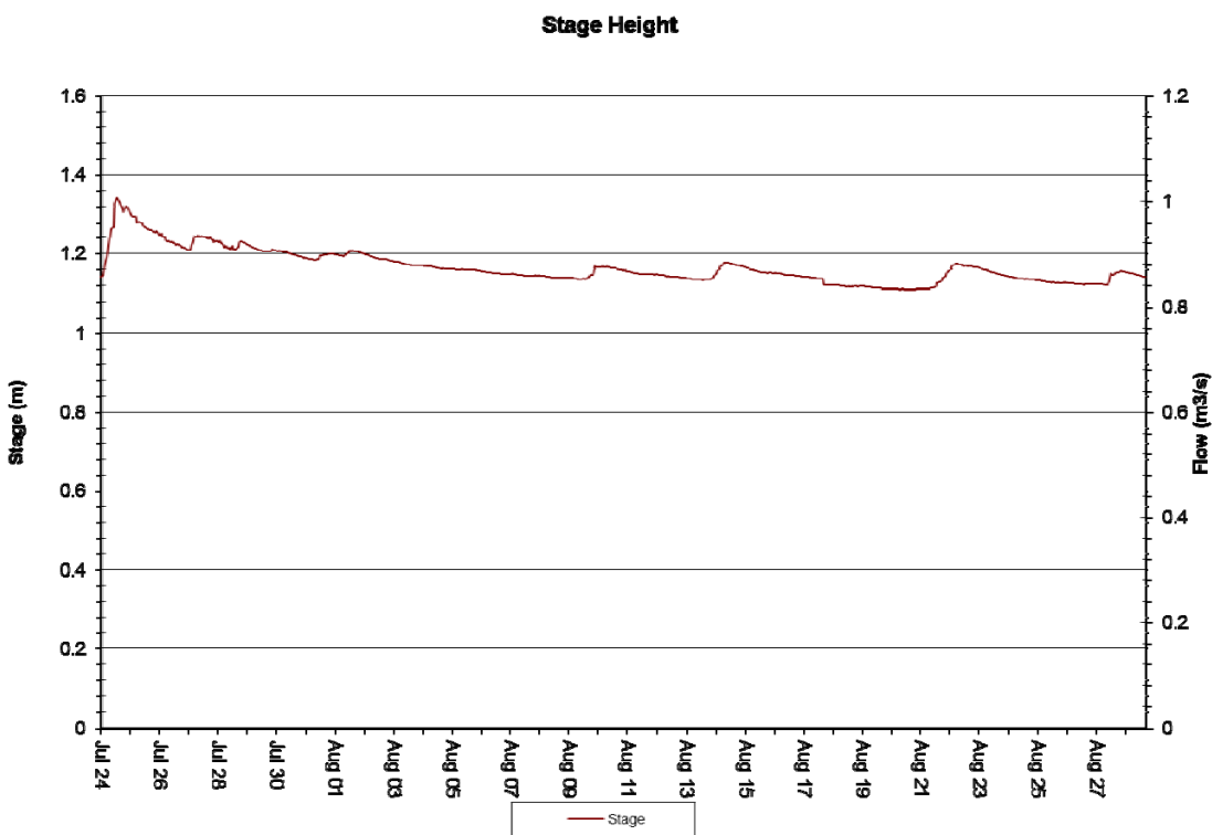
Figure 1: Stage Height (m) at Elross Creek – July 24, 2018 to August 29, 2018
