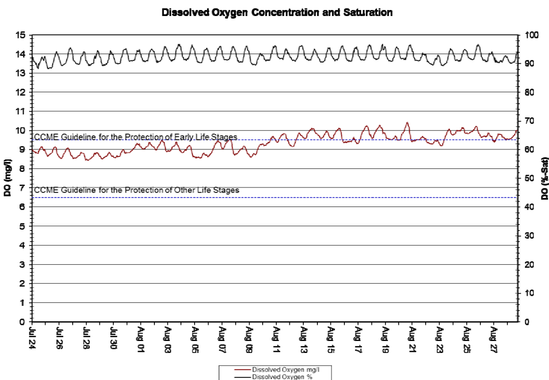
Figure 9: DO (mg/l & % Sat.) at Elross Creek – July 24, 2018 to August 29, 2018
