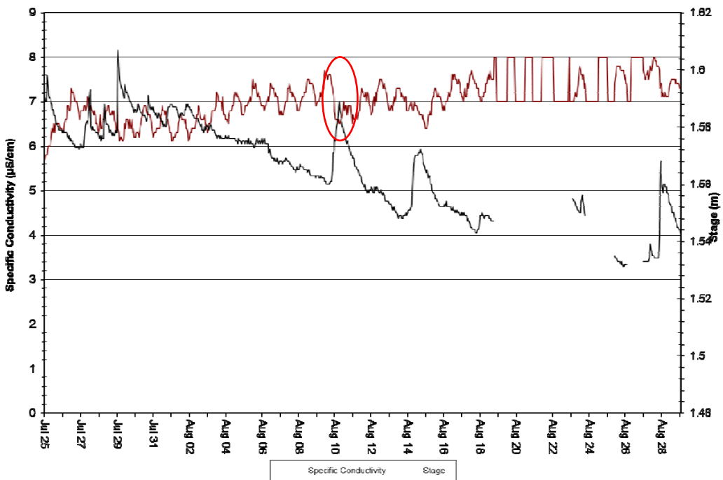
Figure 8: Specific Conductivity at Joan Brook – July 25, 2018 to August 29, 2018
