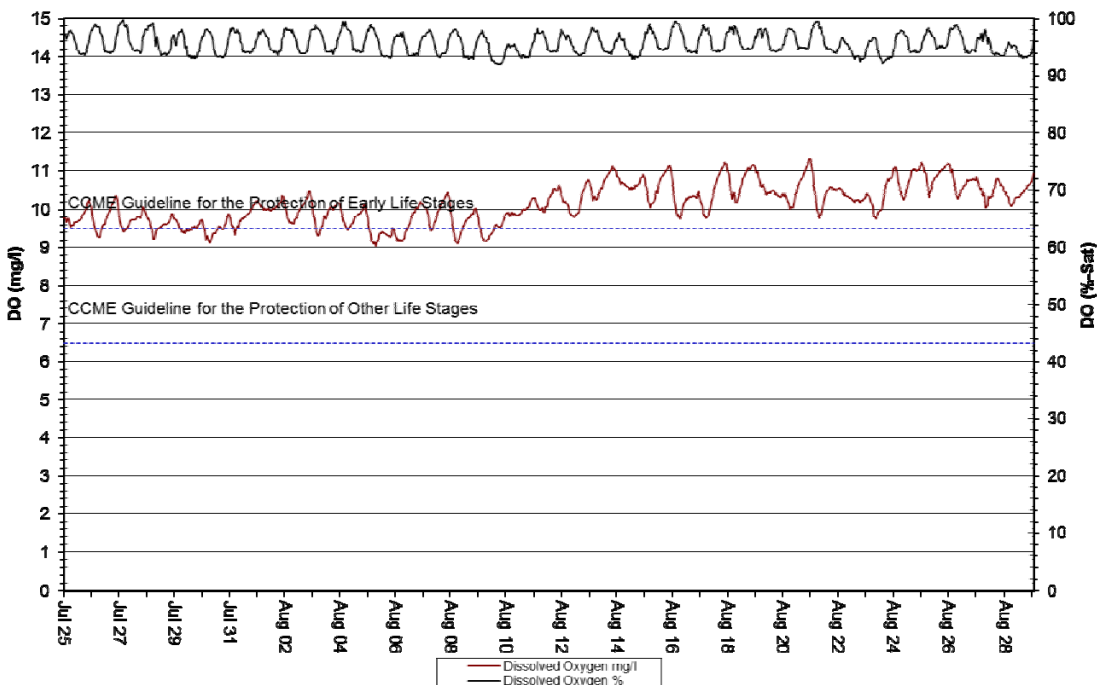
Figure 10: DO (mg/l & % Sat.) at Joan Brook – July 25, 2018 to August 29, 2018
