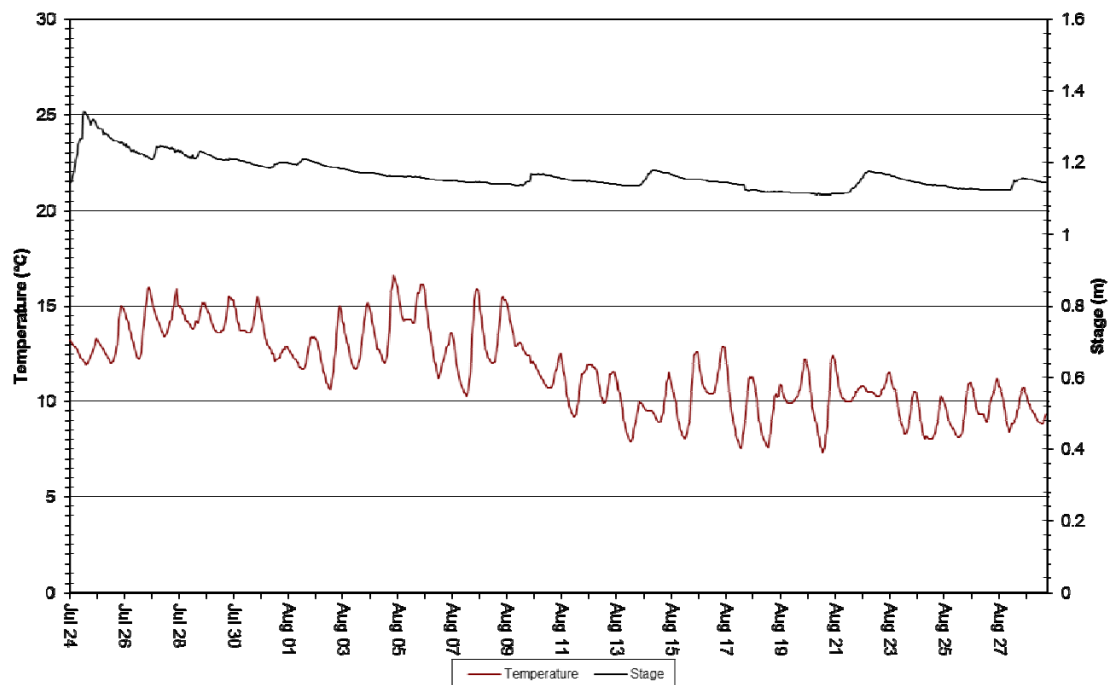
Figure 3: Temperature (°C) - Elross Creek – July 24, 2018 to August 29, 2018
