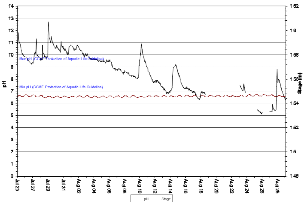
Figure 6: pH at Joan Brook – July 25, 2018 to August 29, 2018
