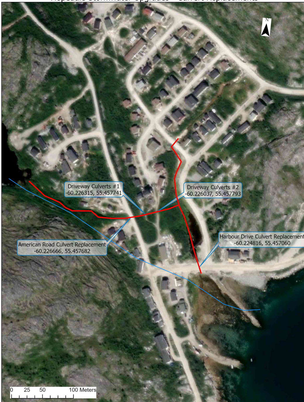
Hopedale Stormwater Upgrades - Culvert Replacements
