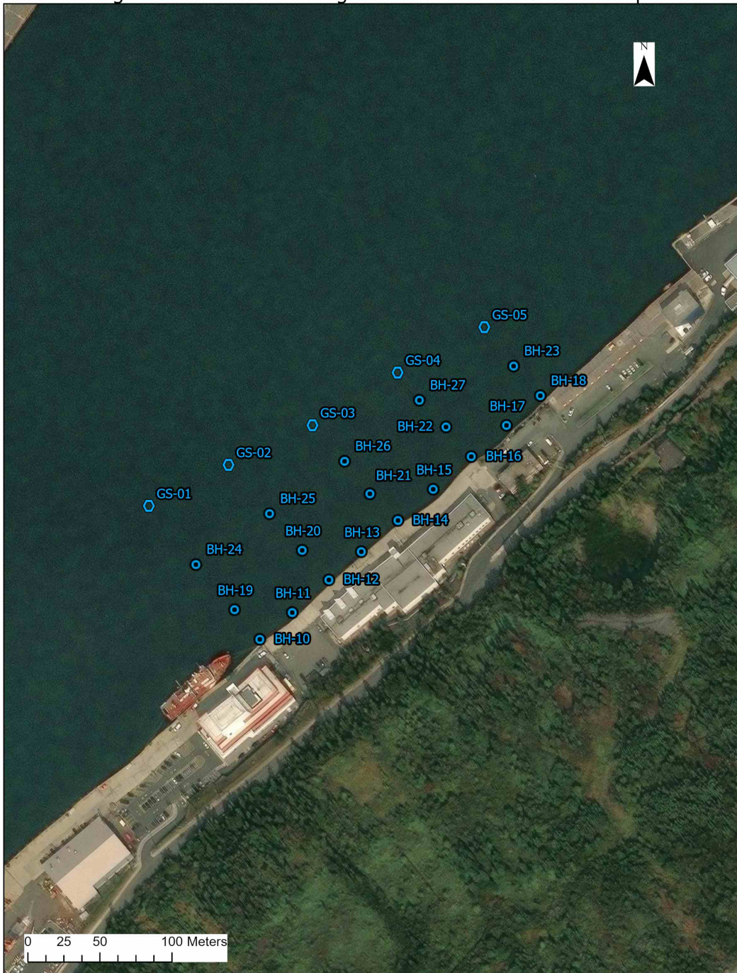
HMCS Berthage - Geotechnical Investigation - Boreholes and Grab Sample Locations
