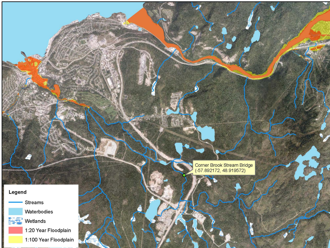
Installation of a Snowmobile/ATV trail bridge across Corner Brook Stream
