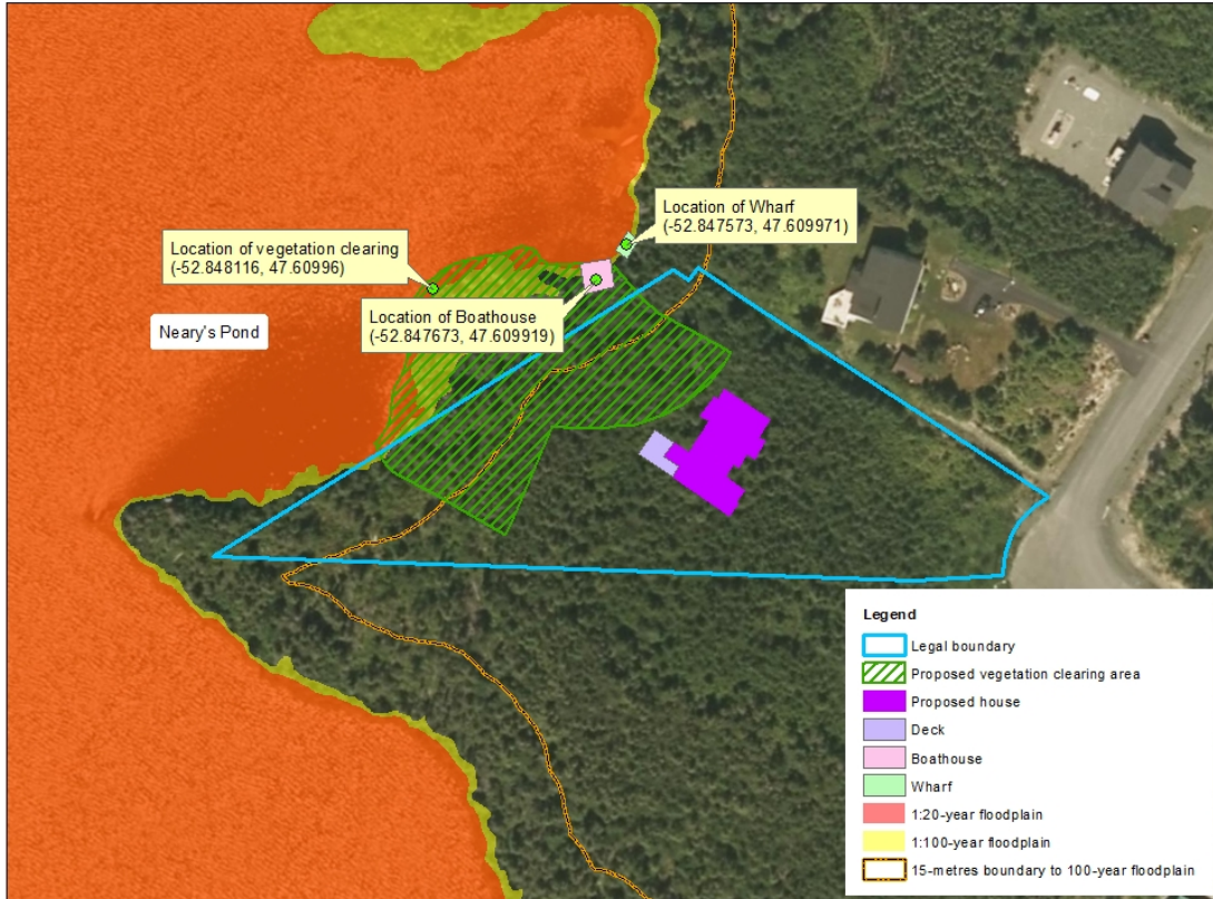
Clearing of vegetation, and construction of Boathouse and Wharf along the shoreline of Neary's Pond 87 Round Pond Road, Portugal Cove-St. Philip's
