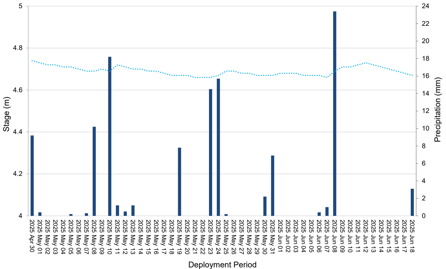
Daily Stage (m) Recorded at John Fitzpatrick RTWQ Station and Total Precipitation (mm) recorded at the St. Lawrence Climate Station.
