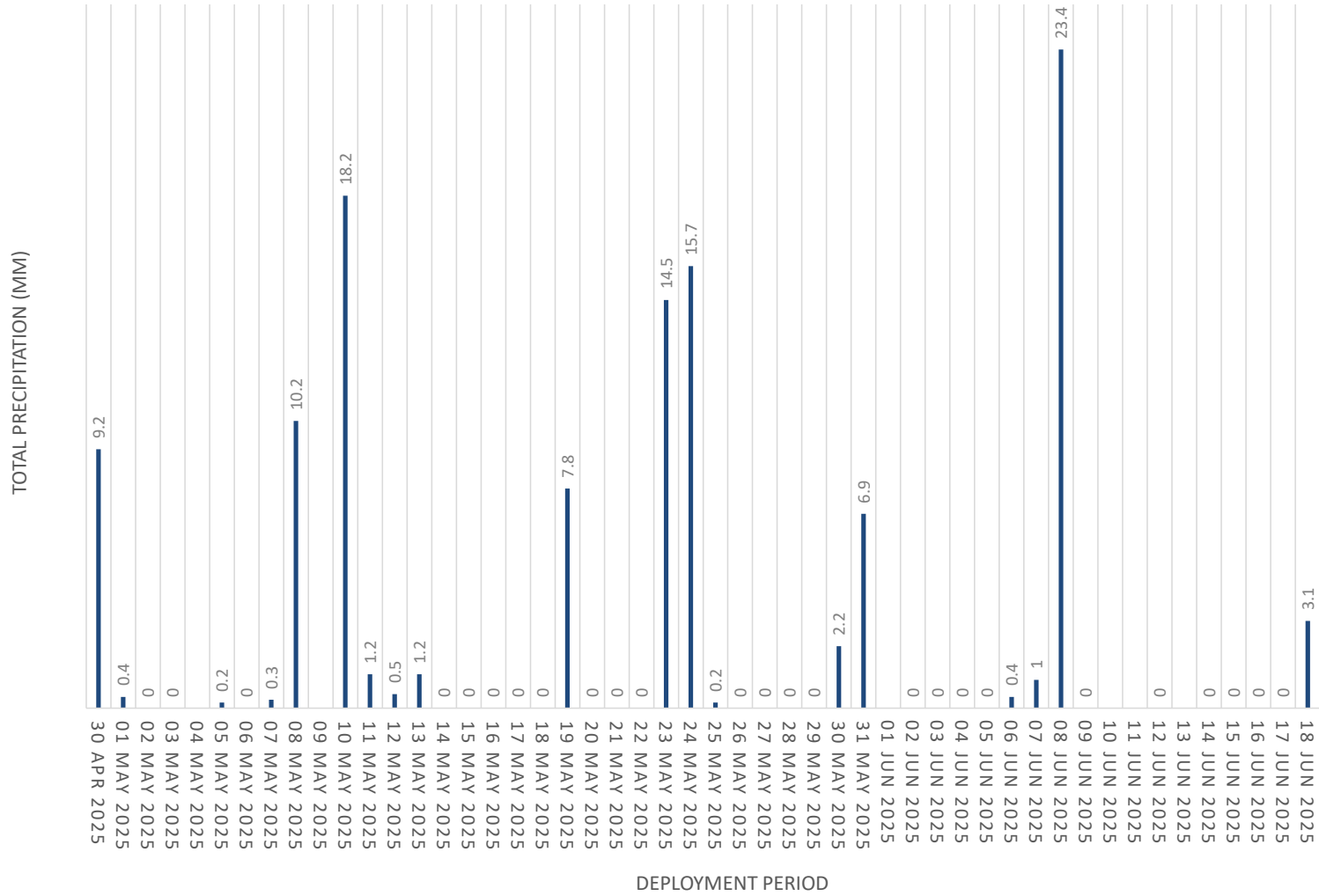
Figure 15: Total Daily Precipitation recorded at the St. Lawrence Environment Canada Weather Station.
