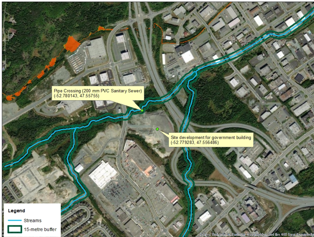
Sanitary Sewer Pipe Crossing across Leary's Brook at 80 Kelsey Drive, St. John's
