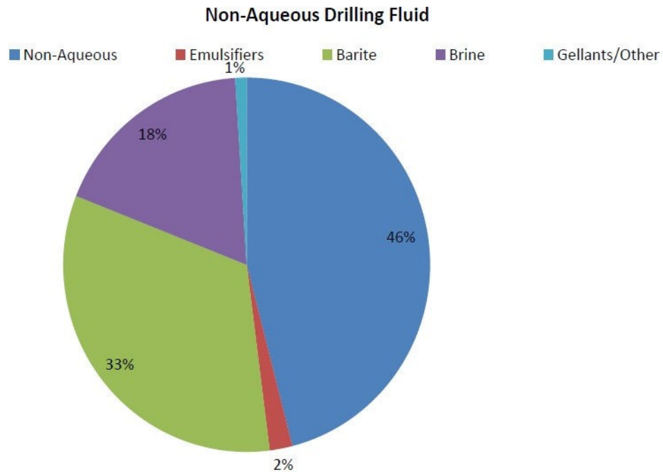
Figure 4-11 Typical Non-Aqueous Drilling Fluid Composition by Volume
