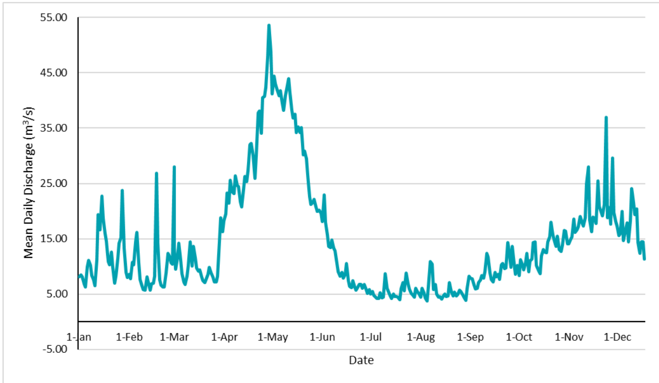
Figure 4-7: Estimated Mean Annual Flow (MAF) based on pro-rated flows from Highlands River station (Station # 02ZA002)
