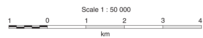
MAP 2001-25 UNTITLED NEWFOUNDLAND
