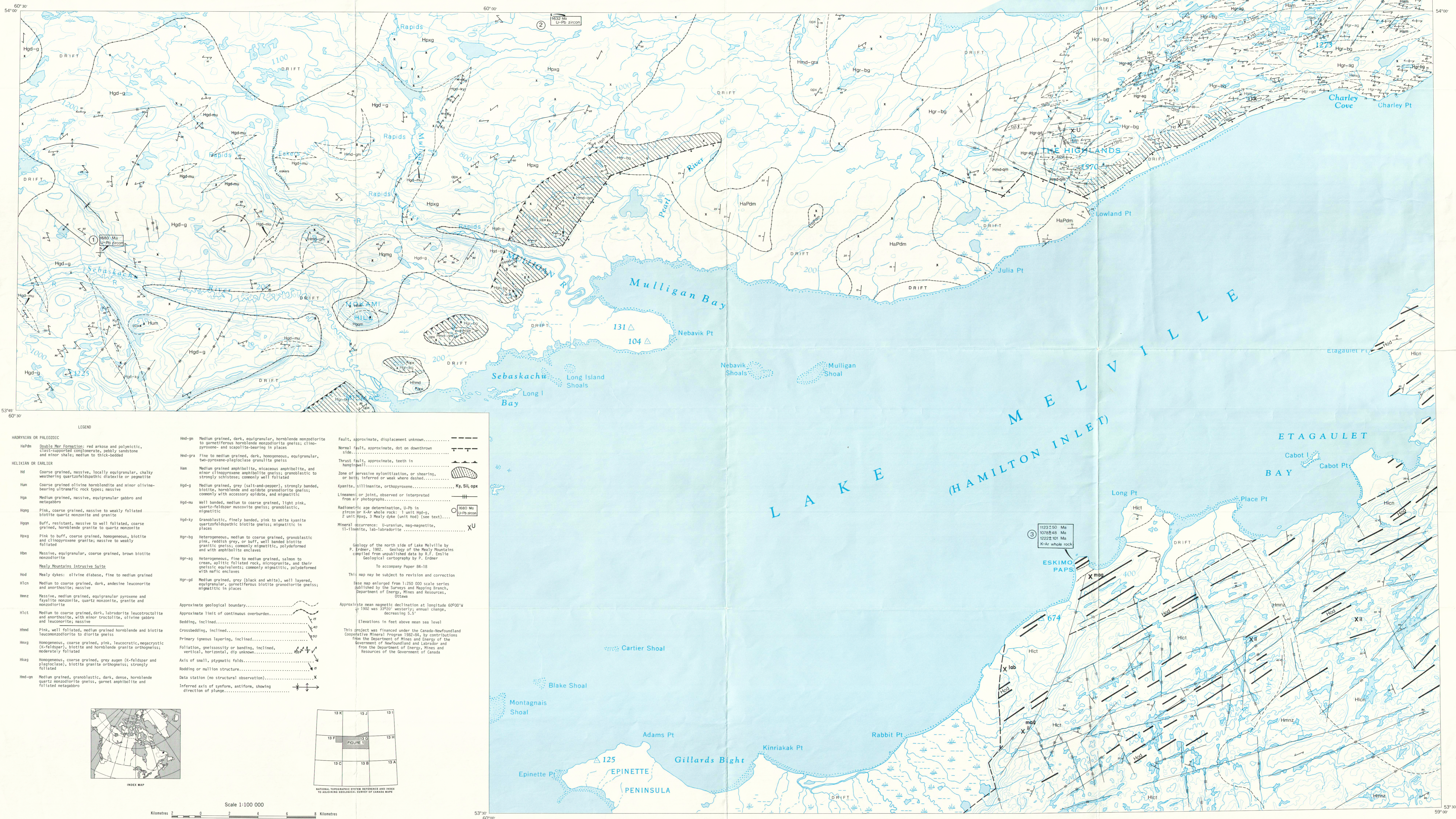
Figure 1. Geology of the Lake Melville-Double Mer area, Labrador
