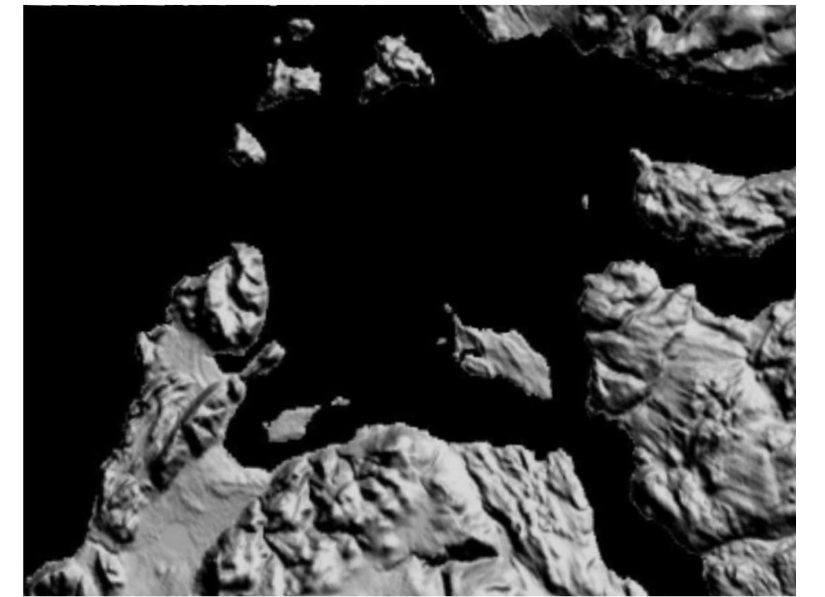
Digital Elevation Model (DEM) from Shuttle Radar Topography Mission (SRTM) data of the Little Grand Lake map area (shaded from the northeast). The image provides additional surface information not readily illustrated on the surficial map. Terrain variability is evident, with areas of bedrock highlighted as higher, rougher textured areas (consistent with surficial map), and areas of thicker till shown as smoother textured areas.
