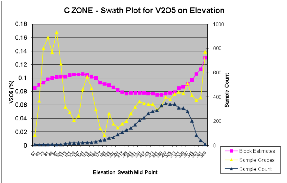
FIGURE 17-6 SWATH PLOT FOR V 2 O 5 SHOWING E-W SLICES THROUGH THE DEPOSIT
