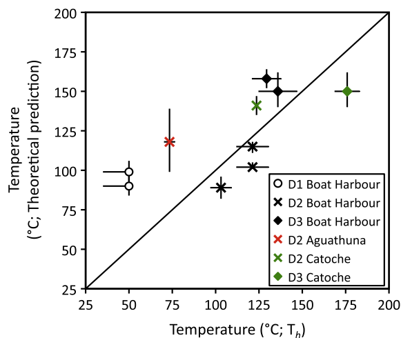
Fig. 5. The relationship between the temperatures derived from fluid inclusion microthermometry ( T_h ) (Azmy et al., 2008, 2009; Conliffe et al., 2009; Azmy and Conliffe, 2010; Azomani et al., 2013; Olanipekun et al., 2014) and the \Delta_{47} temperatures as determined using the theoretical calcite relationship of Schauble et al. (2006) with the intercept of Guo et al. (2009) transferred to the absolute reference frame using the transfer function of Dennis et al. (2011). Open circles represent D1; “x” symbols represent D2; filled diamonds represent D3. Black symbols represent data from the Boat Harbour formation; green symbols represent data from the Catoche formation; red symbols represent data from the Aguathuna formation. The 50 °C values for D1 samples represent maximum temperatures (see Section 3.2). Error bars on fluid inclusions temperature represent 1 standard deviation ( 1\sigma ). Error bars on \Delta_{47} temperatures represent 1 SE uncertainty in \Delta_{47} propagated through the calibration equation. The black line represents a 1:1 relationship. (For interpretation of the references to colour in this figure legend, the reader is referred to the web version of this article.)
