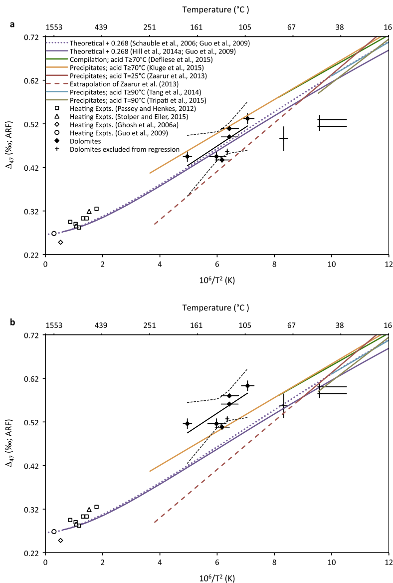
Fig. 6. A comparison of \Delta_{47} data from dolomites (this study) to published calcite calibrations. (A) Data corrected using the phosphoric acid fractionation factor of Defliese et al. (2015). The dotted purple line represents the theoretical calcite relationship of Schauble et al. (2006) with the intercept of Guo et al. (2009) transferred to the absolute reference frame using the transfer function of Dennis et al. (2011). The solid purple line represents the theoretical calcite relationship of Hill et al. (2014a) with the intercept of Guo et al. (2009) transferred to the absolute reference frame using the transfer function of Dennis et al. (2011). The green line represents the calibration of Defliese et al. (2015), which includes calibration data from their study as well as calibration data from previous studies. Data included in the Defliese et al. (2015) compilation are: Eagle et al. (2010), Dennis and Schrag (2010), Dennis et al. (2011), Eagle et al. (2013a), Henkes et al. (2013), Fernandez et al. (2014), and Tang et al. (2014). The orange line represents a least squares linear regression through the synthetic calibration data of Kluge et al. (2015), which we recalculated using the acid fractionation factor of Defliese et al. (2015). The red line represents the calibration of Zaarur et al. (2013), which includes their calibration data from synthetic carbonates as well as calibration data from the synthetic carbonates of Ghosh et al. (2006a). The dashed red line represents an extrapolation of the Zaarur et al. (2013) equation to precipitation temperatures beyond the scope of the authors' sample suite. The blue line represents the calibration of Tang et al. (2014), which we modified to reflect the acid fractionation factor of Defliese et al. (2015). The brown line represents the calibration of Tripathi et al. (2015), which we modified to reflect the acid fractionation factor of Defliese et al. (2015). Open triangles (Stolper and Eiler, 2015), open squares (Passey and Henkes, 2012), the open diamond (Ghosh et al., 2006a) and the open circle (Guo et al., 2009) represent data from calcites used in heating experiments. All dolomite samples from the present study were reacted at 90 °C, and values were converted to 25 °C using a correction of 0.082‰ (Defliese et al., 2015). Error bars on \Delta_{47} represent the standard error of replicate measurements (1 SE). Error bars on temperature ( T_h ) values represent 1 standard deviation (1 \sigma ). Black filled diamonds represent samples from our suite that did not show obvious evidence of solid-state reordering as described in Section 6.1.2; crosses represent samples that did show evidence of solid-state reordering as described in Section 6.1.2. The black line represents a least squares linear regression using the St. George Group data that did not show evidence of solid-state reordering. The dashed black lines represent the 95% confidence interval on that regression. All \Delta_{47} data are reported on the absolute reference frame (ARF) of Dennis et al. (2011). (B) As in (A), except with the dolomite data from the present study corrected using the phosphoric acid fractionation factor of Murray et al. (2016). (For interpretation of the references to colour in this figure legend, the reader is referred to the web version of this article.)
