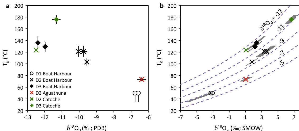
Fig. 3. Previously published fluid inclusion temperatures ( T_h ) of dolomite cements (Azmy et al., 2008, 2009; Conliffe et al., 2009; Azmy and Conliffe, 2010; Azomani et al., 2013; Olanipekun et al., 2014) and newly acquired oxygen isotopic measurements. (A) Mean \delta^{18}\text{O}_d (PDB) plotted versus T_h ; (B) calculated \delta^{18}\text{O}_w (SMOW) versus T_h . The \delta^{18}\text{O}_w values were calculated using \delta^{18}\text{O}_d , the previously published T_h values, and the equation of Horita (2014). Contours of \delta^{18}\text{O}_d are derived from a published calibration for dolomite (Horita, 2014). Error bars in (A) represent 1 standard deviation on T_h and \delta^{18}\text{O}_d . Shaded error spaces in (B) represent the 1 \sigma range of possible T_h values and the 1 \sigma uncertainty in \delta^{18}\text{O} propagated through the calibration equation. Open circles represent D1; “x” symbols represent D2; filled diamonds represent D3. Black symbols represent data from the Boat Harbour formation; green symbols represent data from the Catoche formation; red symbols represent data from the Aguathuna formation. The 50 °C values for D1 samples represent maximum temperatures (see Section 3.2). (For interpretation of the references to colour in this figure legend, the reader is referred to the web version of this article.)
