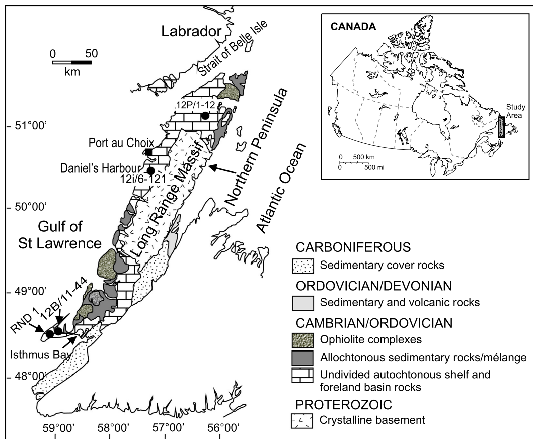
Fig. 1. A map of the study area showing the locations of sampled outcrops and cores, which represent the Lower Ordovician St. George Group carbonates in western Newfoundland, Canada (Knight et al., 2008; Azomani et al., 2013).
