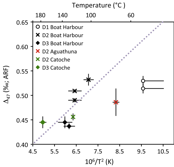
Fig. 4. The relationship between the \Delta_{47} of dolomites (this study) and previously published fluid inclusion temperatures ( T = T_h ). Dolomites were reacted at 90 °C, and \Delta_{47} values were converted to 25 °C using a correction of 0.082‰ (Defliese et al., 2015). All \Delta_{47} data are reported on the absolute reference frame (ARF) of Dennis et al. (2011). Error bars on \Delta_{47} represent the standard error of replicate measurements (1 SE). Error bars on temperature values ( T_h ) represent 1 standard deviation (1 \sigma ). Open circles represent D1; “x” symbols represent D2; filled diamonds represent D3. Black symbols represent data from the Boat Harbour formation; green symbols represent data from the Catoche formation; red symbols represent data from the Aguathuna formation. The 50 °C values for D1 samples represent maximum temperatures (see Section 3.2). The dotted purple line represents the theoretical calcite relationship as determined by Schauble et al. (2006) with the intercept of Guo et al. (2009) transferred to the absolute reference frame using the transfer function of Dennis et al. (2011). (For interpretation of the references to colour in this figure legend, the reader is referred to the web version of this article.)
