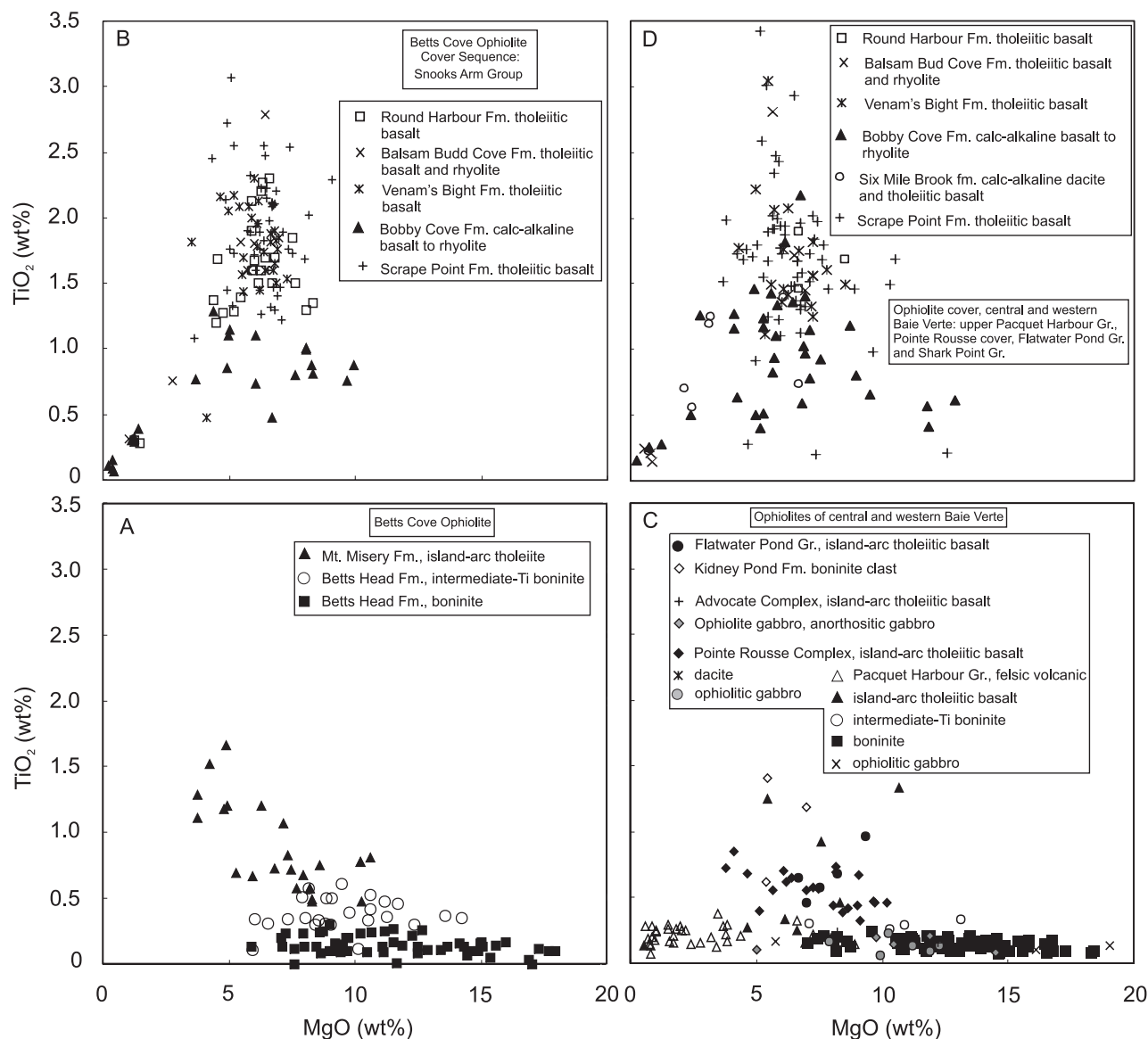
Figure 4. \text{TiO}_2 versus \text{MgO} diagram. A) Volcanic rocks of the Betts Head and Mount Misery formations, Betts Cove Complex. Data from Bédard (2000b) and references therein. B) Volcanic rocks of the Snooks Arm Group (see A for data sources). C) Ophiolite-related, boninites and island-arc tholeiitic rocks of the southern Pacquet Harbour Group, Point Rousse Complex, Flatwater Pond Group and Advocate Complex. Data from this study, Gale (1971), Kambampati (1984) and Piercey (1996). D) Ophiolite volcanic cover of the Pacquet Harbour Group, Point Rousse cover sequence, Flatwater Pond Group and Shark Point Group (see data sources from C above).
