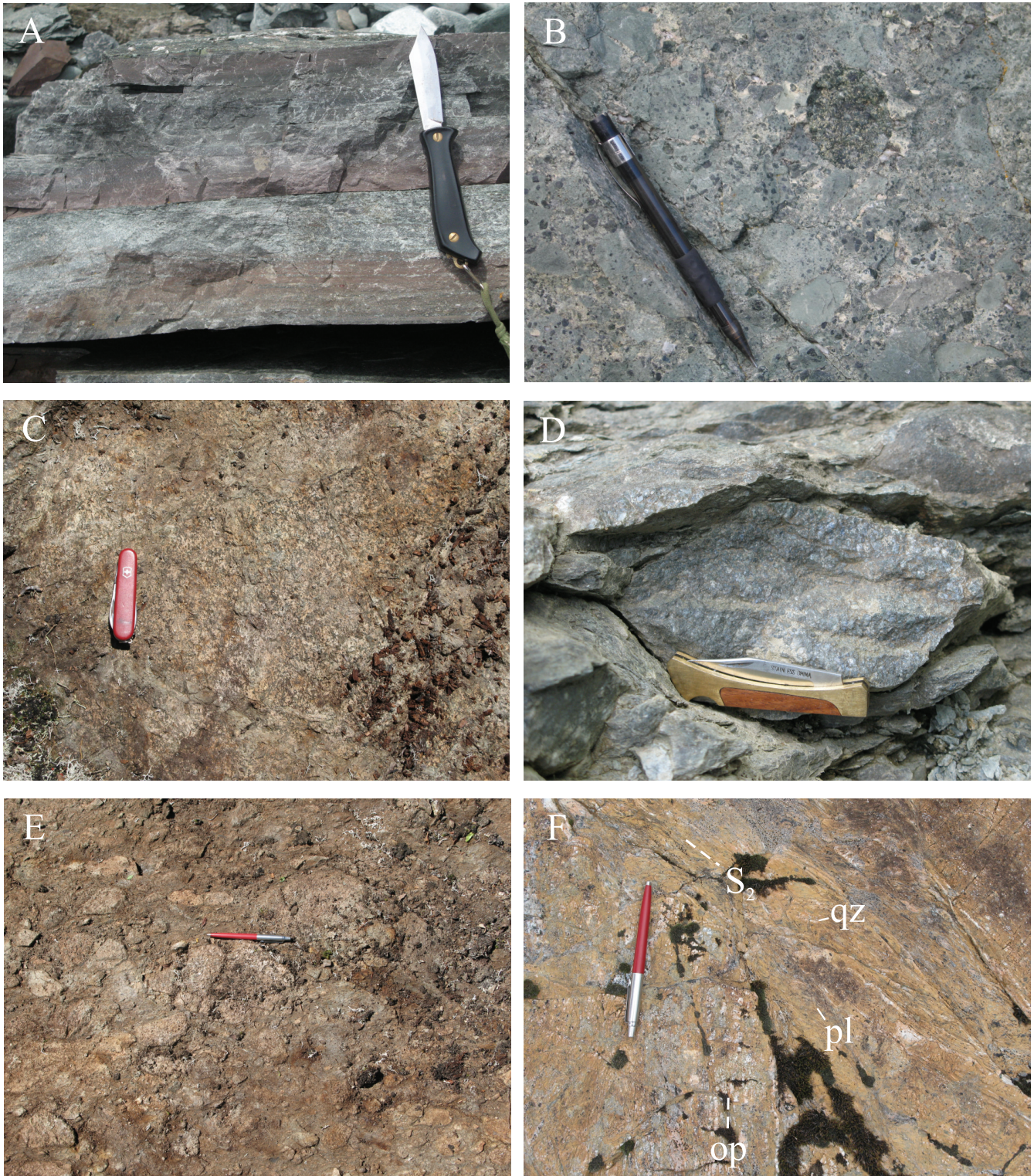
Plate 3. A) Photo of Goldenville horizon, base of Point Rousse cover sequence showing magnetite iron formation, red argillite and green wacke beds. B) Photo of clinopyroxene-phyric tuff breccia with clinopyroxenite cognate xenoliths, Point Rousse cover sequence. C) Photo of ophiolite-derived, flaser gabbro boulder clast, lower Flatwater Pond Group. D) Photo of a quartzite clast, Kidney Pond formation, Flatwater Pond Group. E) Photo of granodiorite pebbles (dated at 479 Ma nearby) in polymict conglomerate, Kidney Pond formation. F) Photo of mantle harzburgite, Advocate Complex west of Flatwater Pond showing primary orthopyroxene fabric (op) and crosscutting S_2 shear zone; qz - quartz; pl - plagioclase.
