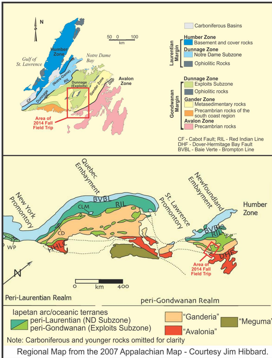
Figure 1. Subdivisions of the Appalachian Orogen in Newfoundland, Atlantic Canada and the adjacent USA, showing the context of the field trip area.
