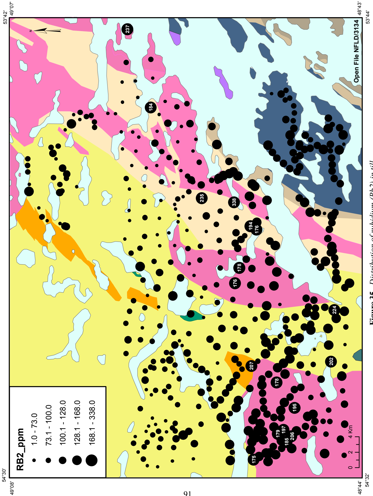
Figure 35. Distribution of rubidium (Rb2) in till.
