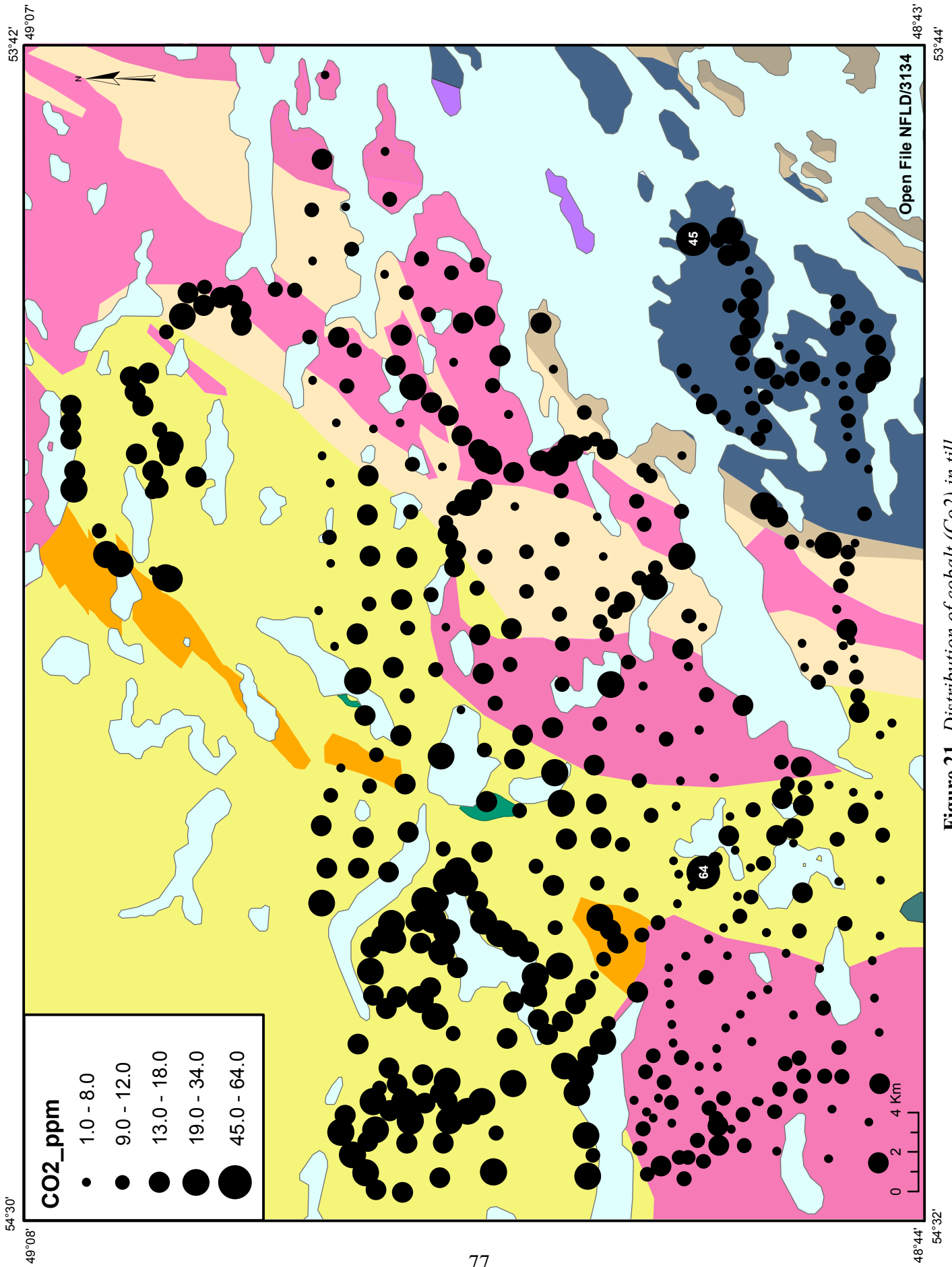
Figure 21. Distribution of cobalt (Co 2 ) in till.
