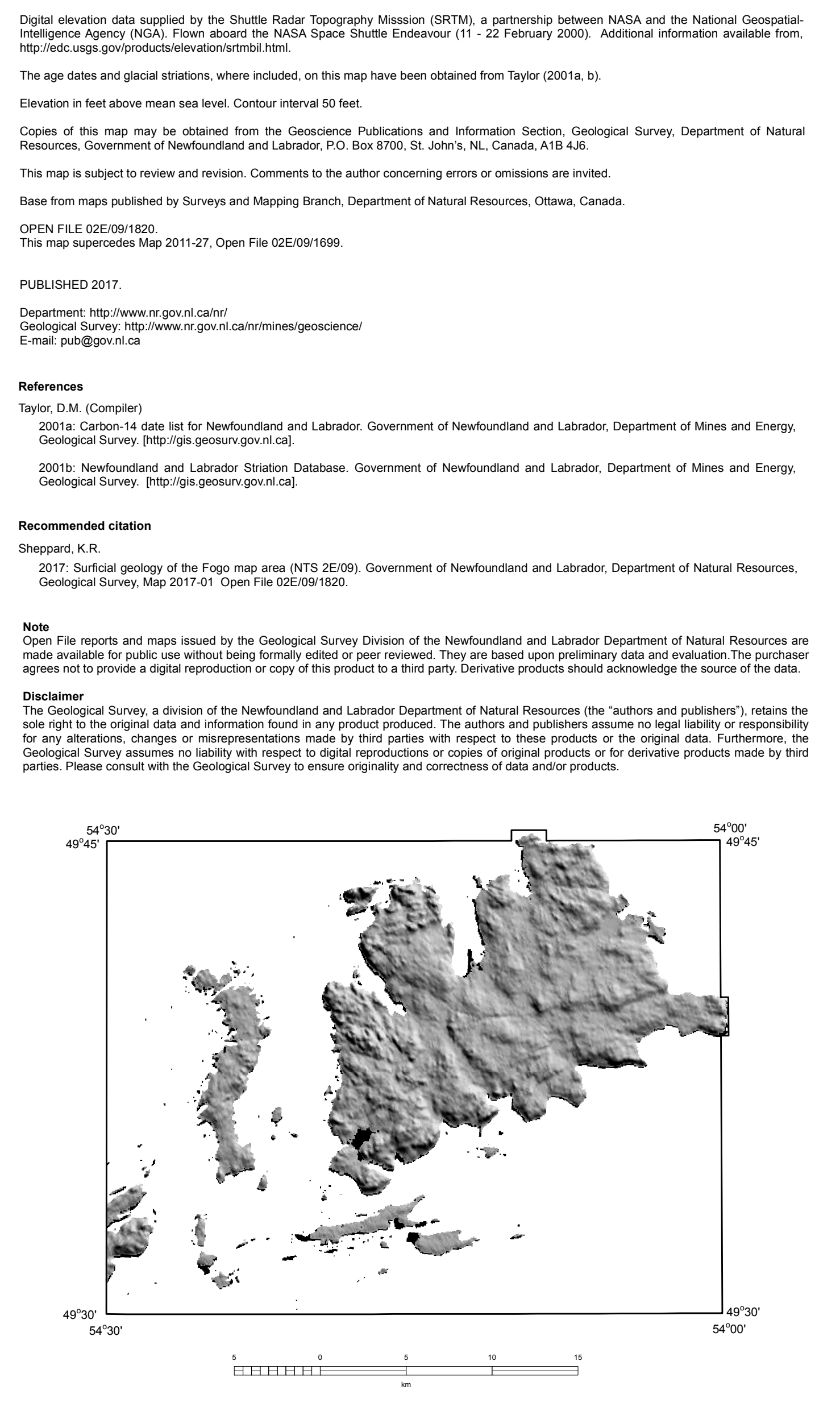
Digital Elevation Model (DEM) from Shuttle Radar Topography Mission (SRTM) of the Fogo map area (shaded from the northeast). The image varies surface information not readily illustrated on the surficial map. Terrain variability is evident, with areas of bedrock highlighted as rougher textured areas (consistent with surficial map), and areas of thicker till shown as smoother textured areas.
