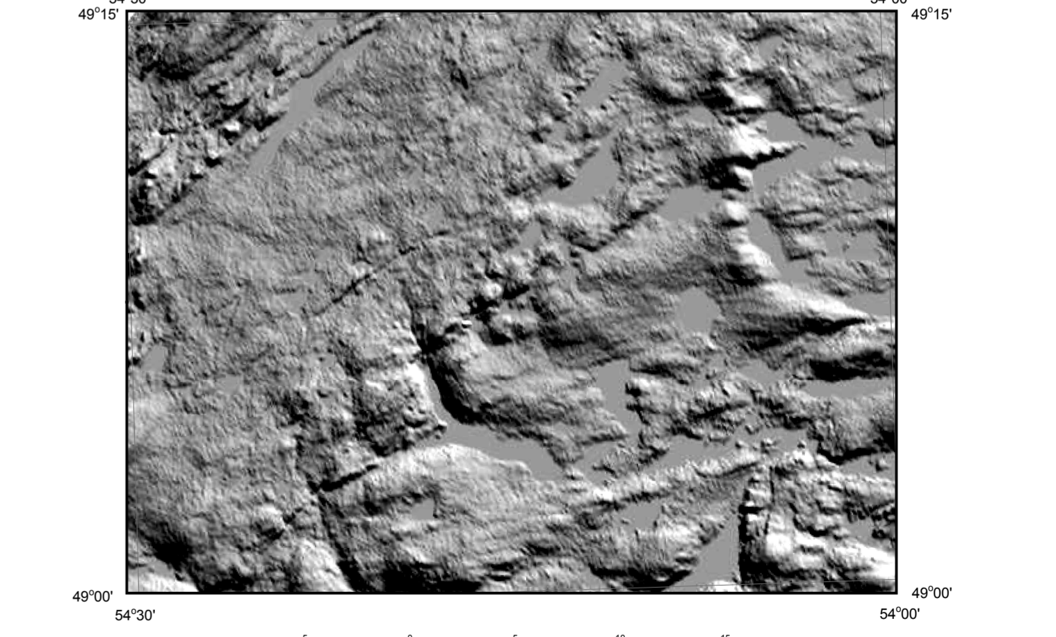
Digital Elevation Model (DEM) from Shuttle Radar Topography Mission (SRTM) data of the Weir's Pond map area (shaded from the northeast). The image provides surface information not readily illustrated on the surficial map. Terrain variability is evident, with areas of bedrock highlighted as rougher textured areas (consistent with surficial map), and areas of thicker till shown as smoother textured areas.
