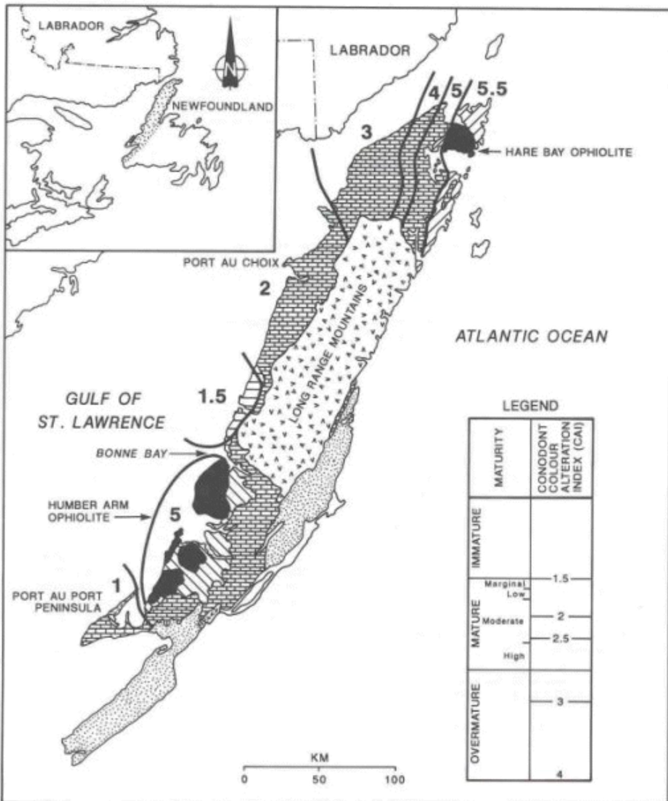
Figure 8. Conodont colour alteration index (CAI) isotherm map for the Ordovician strata of western
