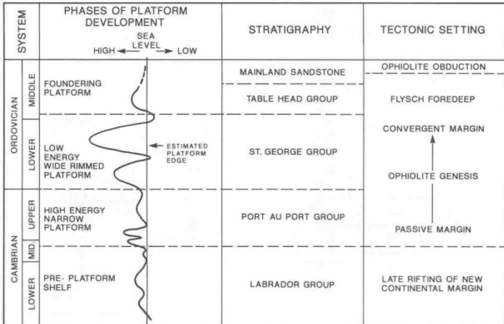
Figure 5. The phases, stratigraphy and tectonic setting of the platform development in the Humber
