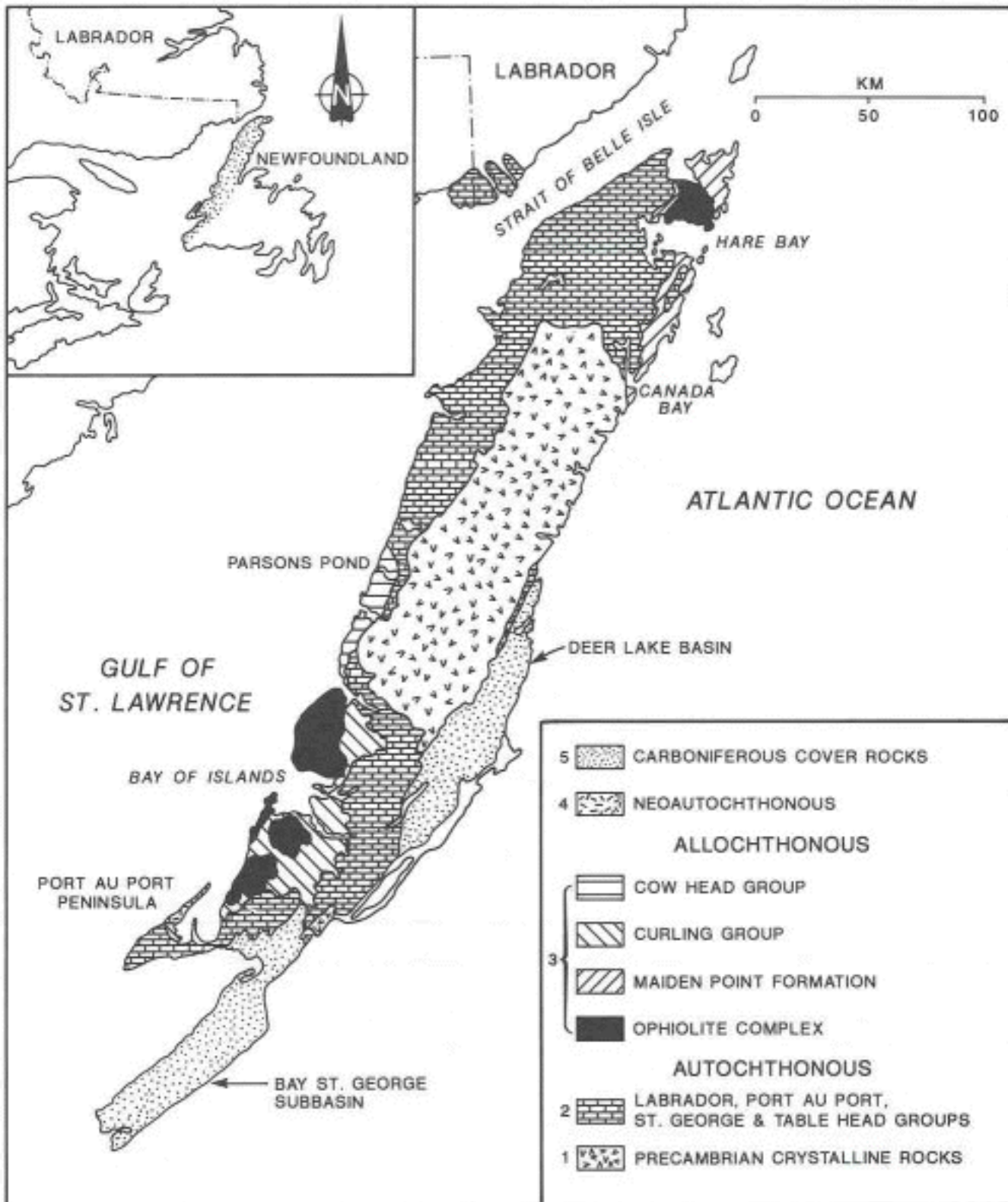
Figure 3. Geological map of Humber Zone in western Newfoundland (after James and Stevens, 1986).
