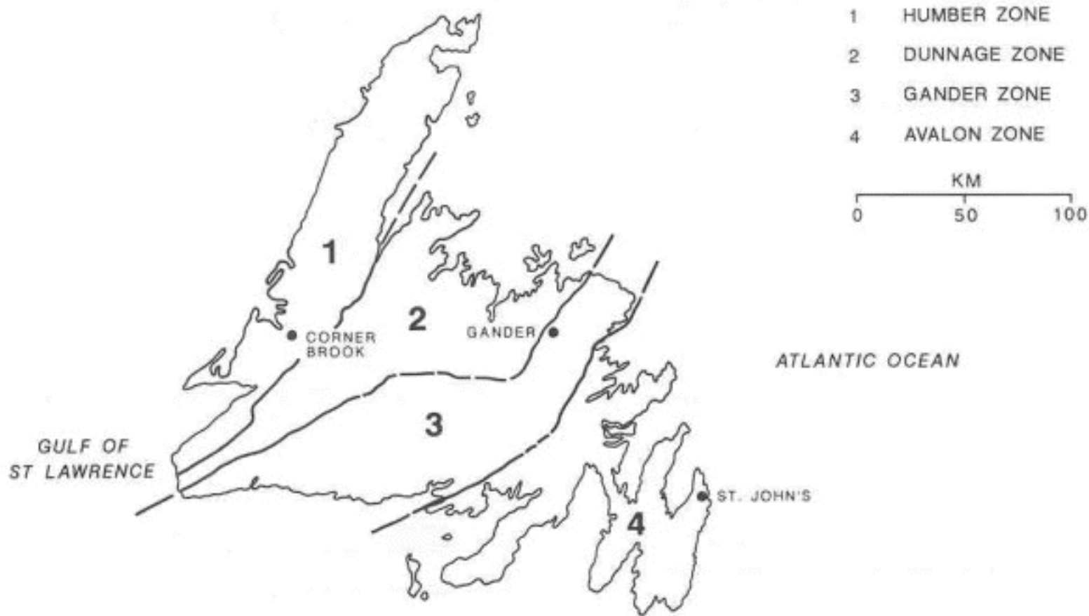
Figure 2. Tectonostratigraphic zones in Newfoundland (after Williams, 1979).
