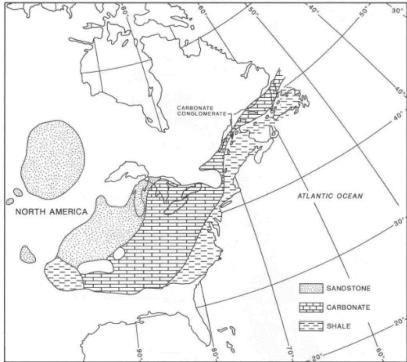
Figure 4. Early Middle Ordovician sedimentary facies covering the eastern margin of ancient North America
