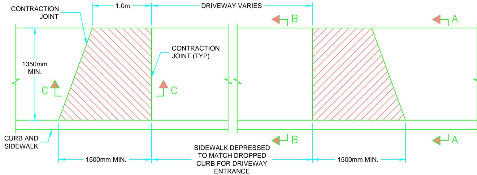
SIDEWALK AT DRIVEWAY ENTRANCE - PLAN
