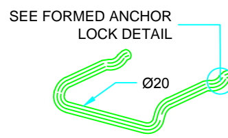
AUXILIARY VIEW
